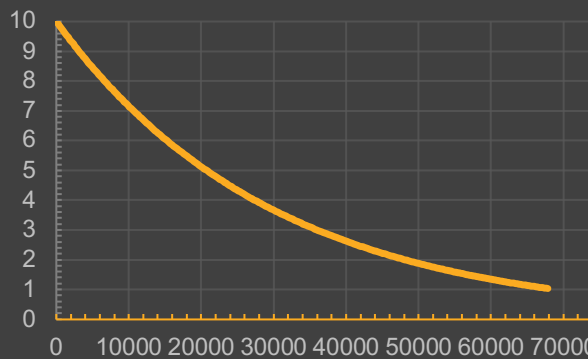
Pipeline Pillow Thickness [Inch] vs Pipe weight [lbs]
